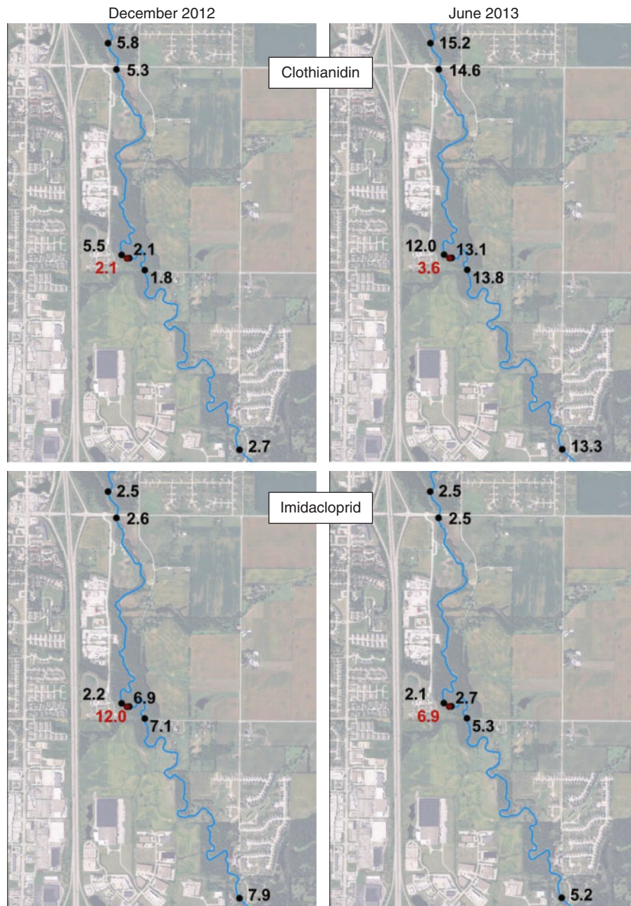
Fig. 7. Concentrations ( \text{ng L}^{-1} ) of clothianidin and imidacloprid collected along Fourmile Creek near Ankeny, Iowa, at two sampling times, December 2012 and June 2013. The concentrations in red are those found at the outfall of the wastewater treatment plant (WWTP).
