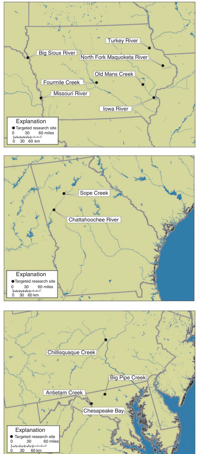
Fig. 2. Sites sampled as part of targeted research studies: elevated hydrologic conditions and in-stream transport in an intense agricultural region in Iowa (a); urban streams in the south-eastern USA (b); and Chesapeake Bay (c).
