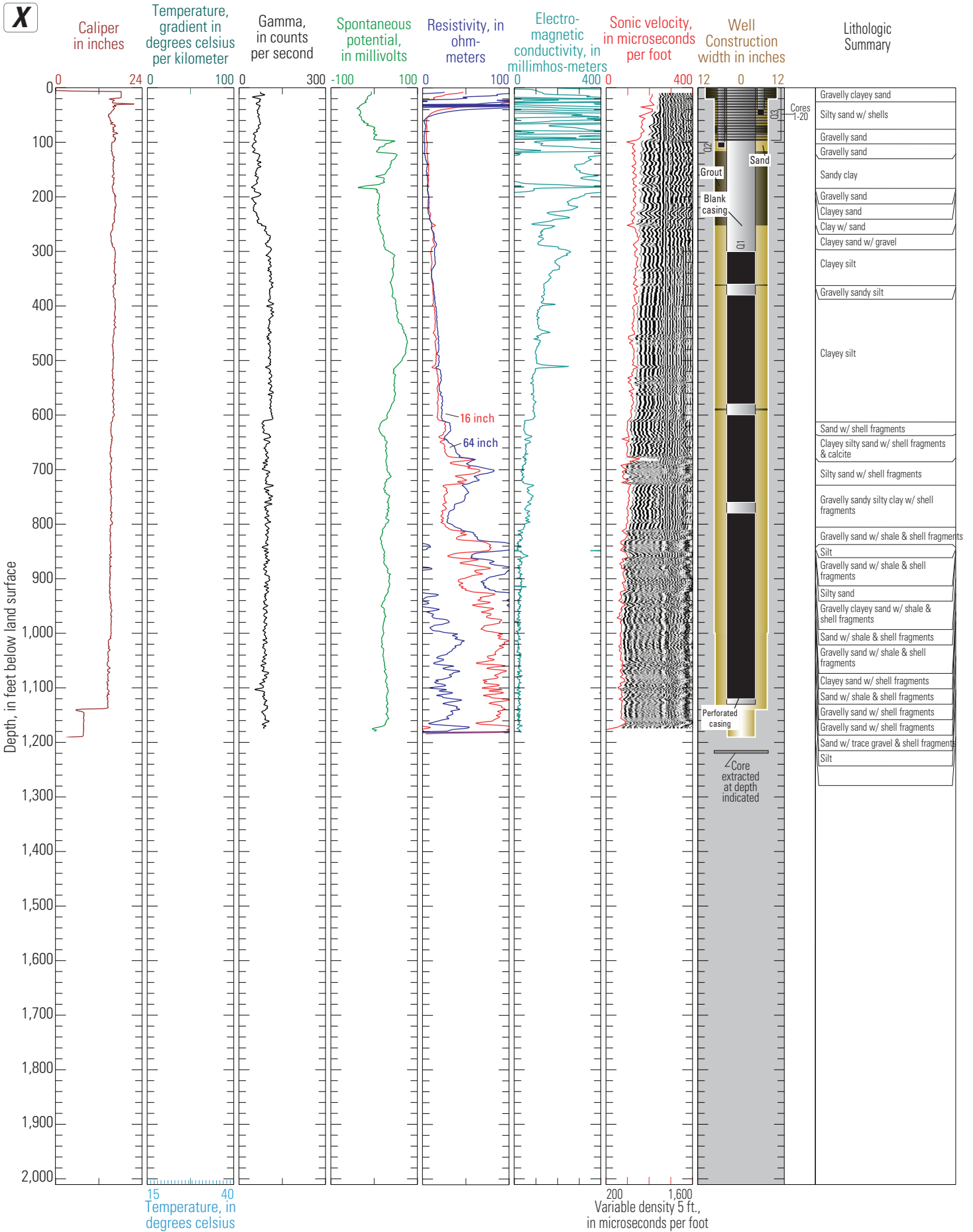
Figure 1X. Well construction diagrams and geophysical log data for caliper, temperature, natural gamma, SP, resistivity, EM, and sonic logs collected from the USGS multiple-depth monitoring-well sites in San Diego County, California, 2009-2013: (A) SDCC (B) SDSW (C) SDHF (D) SDCP (E) SDLH (F) SDSY (G) SDCD.—Continued
