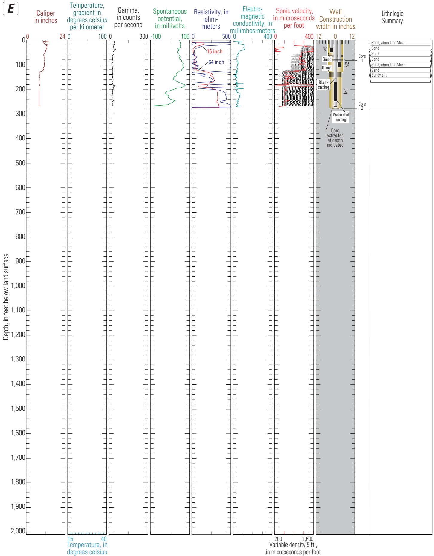
Figure 1E. Well construction diagrams and geophysical log data for caliper, temperature, natural gamma, SP, resistivity, EM, and sonic logs collected from the USGS multiple-depth monitoring-well sites in San Diego County, California, 2009-2013: (A) SDCC (B) SDSW (C) SDHF (D) SDPC (E) SDLH (F) SDSY (G) SDCD.—Continued
