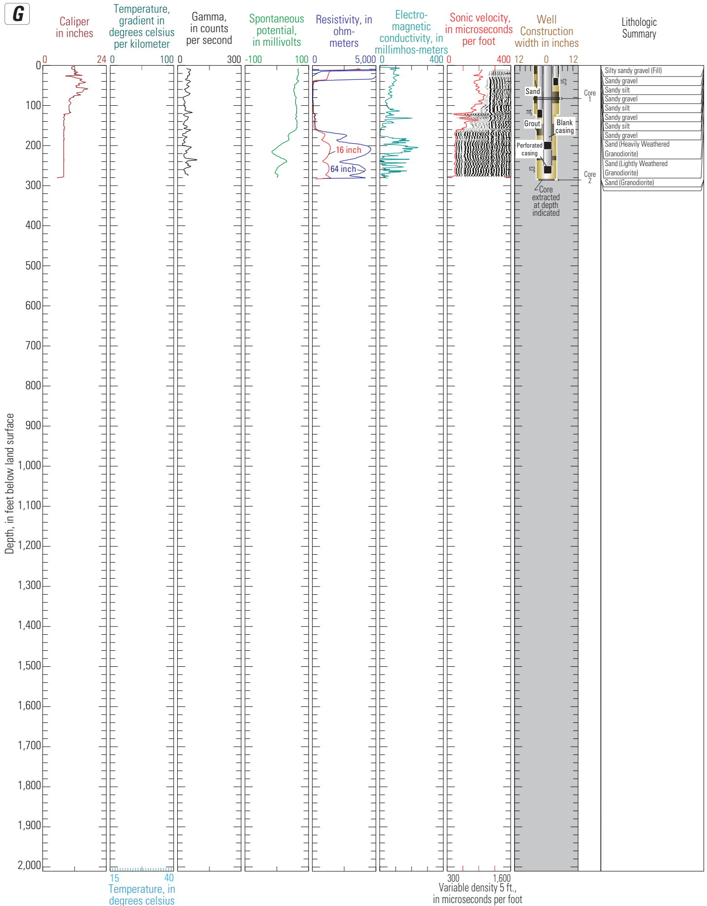
Figure 1G. Well construction diagrams and geophysical log data for caliper, temperature, natural gamma, SP, resistivity, EM, and sonic logs collected from the USGS multiple-depth monitoring-well sites in San Diego County, California, 2009-2013: (A) SDCC (B) SDSW (C) SDHF (D) SDPC (E) SDLH (F) SDSY (G) SDCD.—Continued
