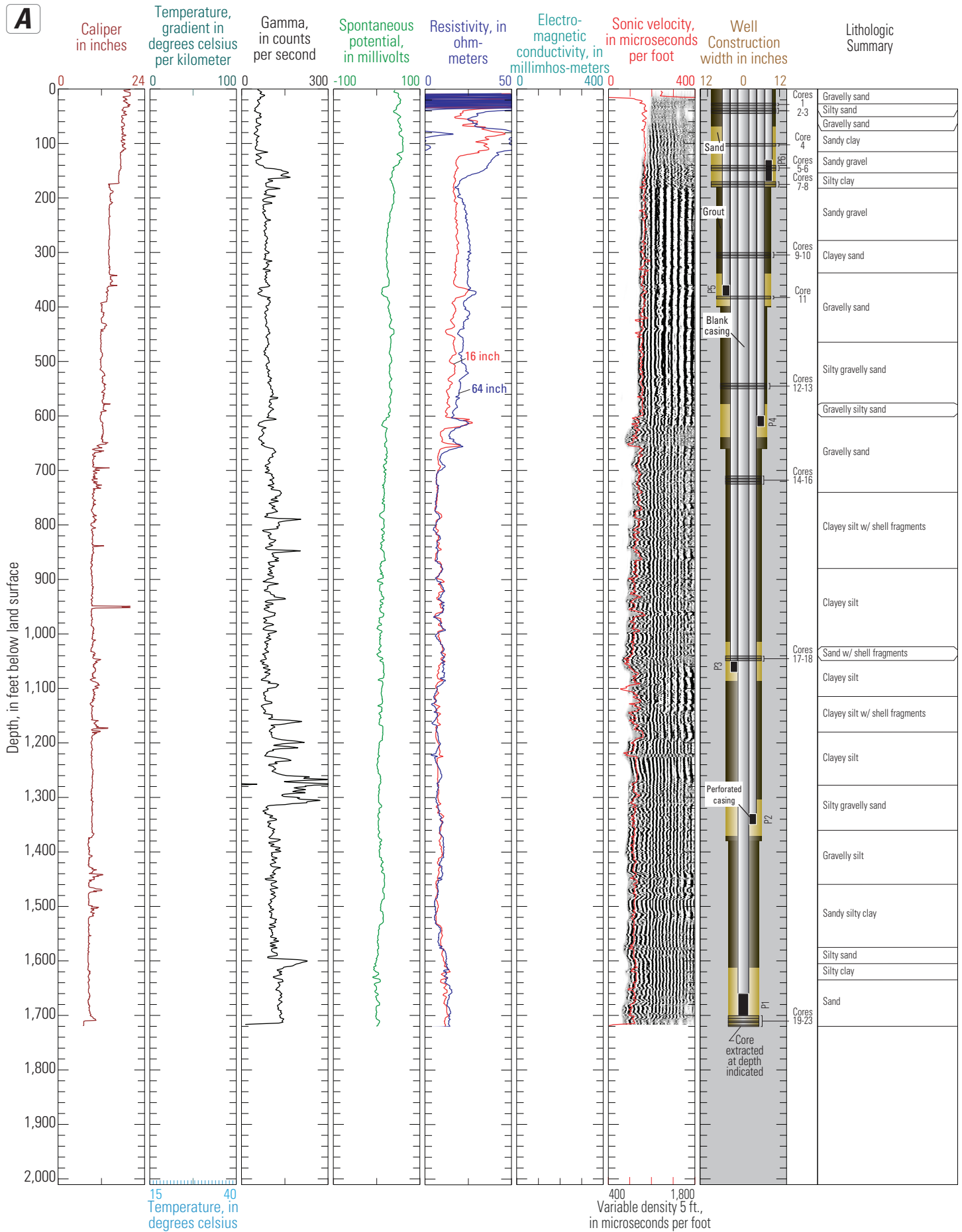
Figure 1A. Well construction diagrams and geophysical log data for caliper, temperature, natural gamma, SP, resistivity, EM, and sonic logs collected from the USGS multiple-depth monitoring-well sites in San Diego County, California, 2009-2013: (A) SDCC (B) SDSW (C) SDHF (D) DDCP (E) SDLH (F) SDSY (G) SDCD.
