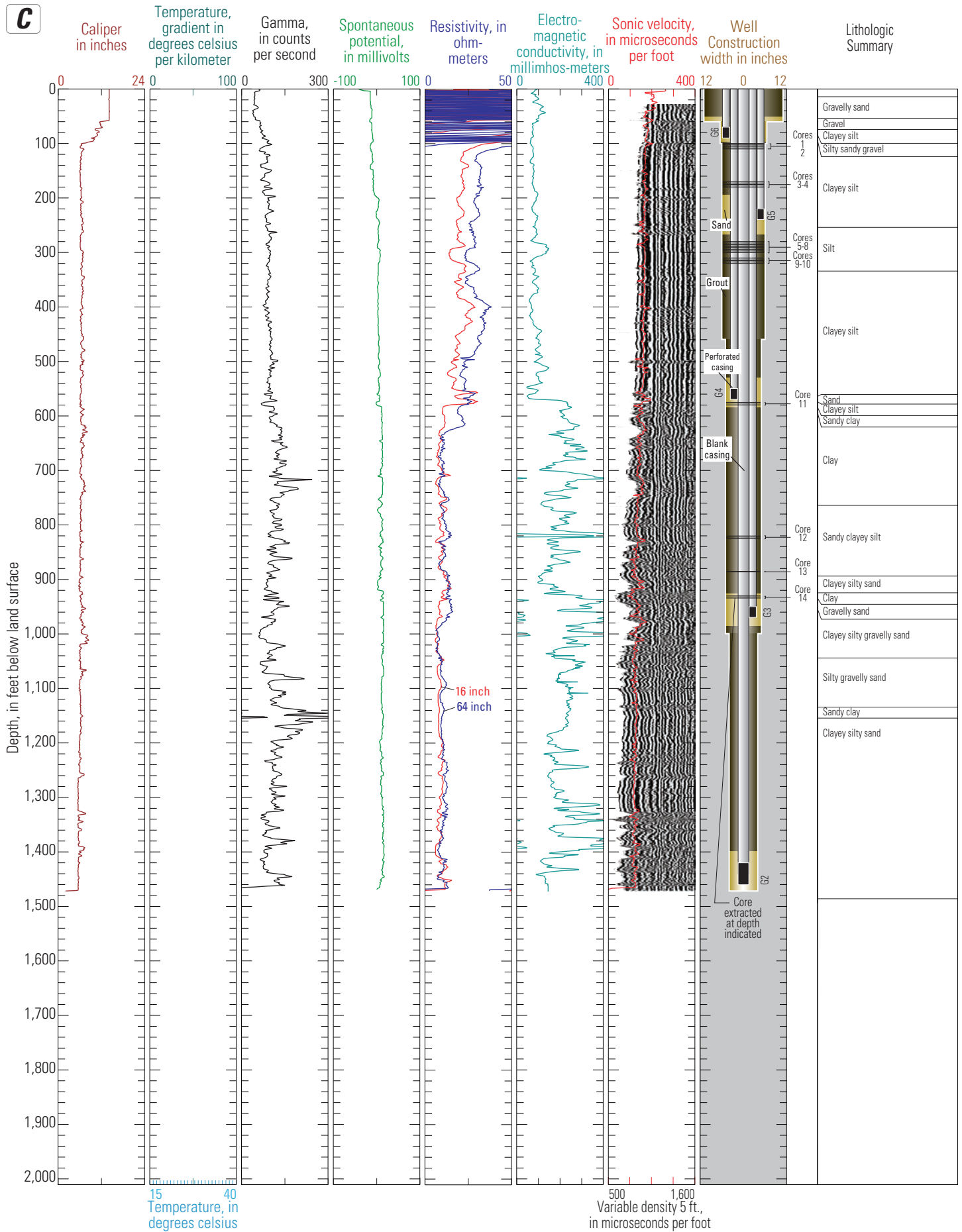
Figure 9C. Well construction diagrams and geophysical log data for caliper, temperature, natural gamma, SP, resistivity, EM, and sonic logs collected from the USGS multiple-depth monitoring-well sites in San Diego County, California, 2003-2009: (A) SDBW (B) SDOT (C) SDOR (D) SDMC (E) SDNB (F) SDEP (G) SDBP (H) SDAQ.—Continued
