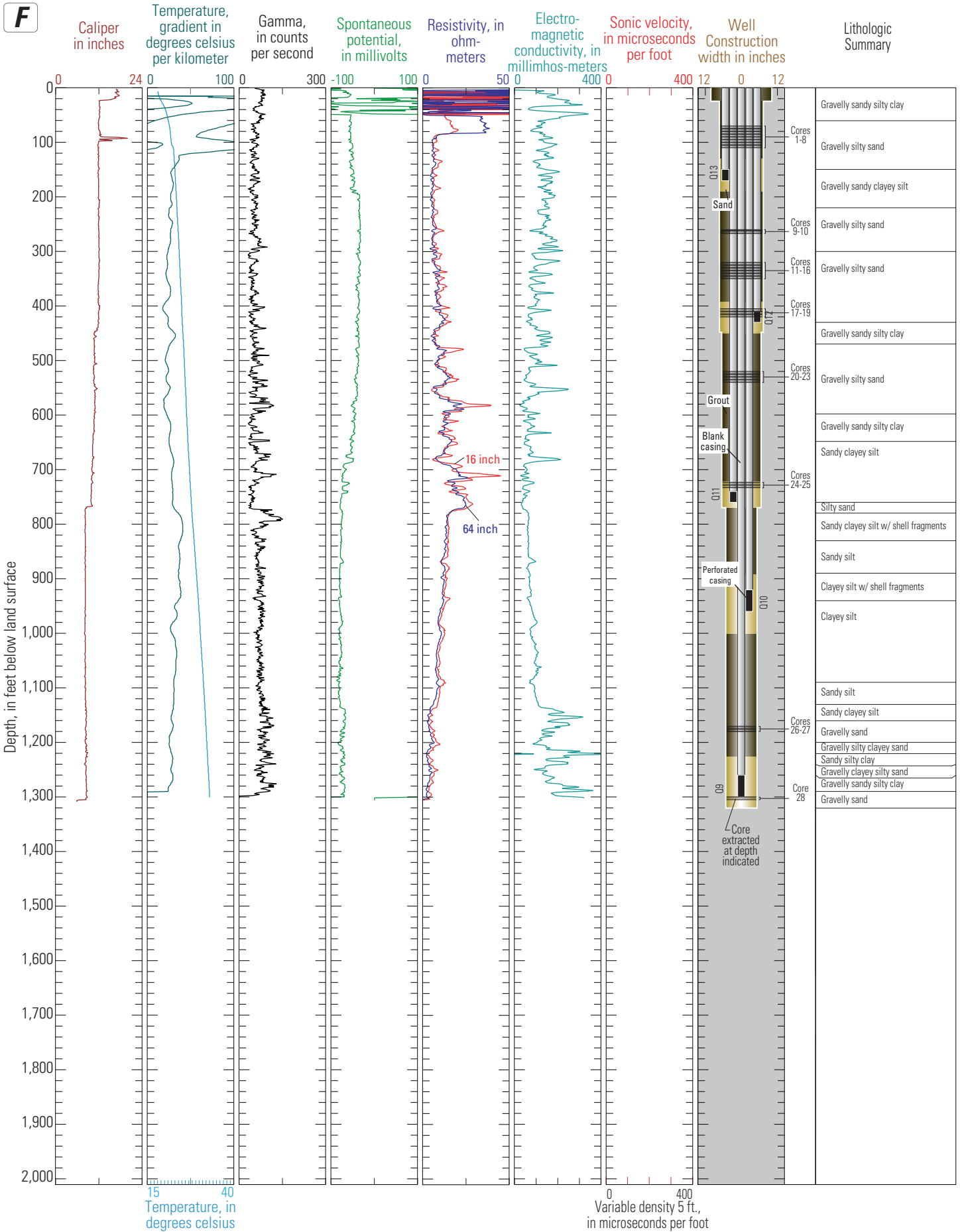
Figure 9F. Well construction diagrams and geophysical log data for caliper, temperature, natural gamma, SP, resistivity, EM, and sonic logs collected from the USGS multiple-depth monitoring-well sites in San Diego County, California, 2003-2009: (A) SDBW (B) SDOT (C) SDOR (D) SDMC (E) SDNB (F) SDEP (G) SDBP (H) SDAQ.—Continued
