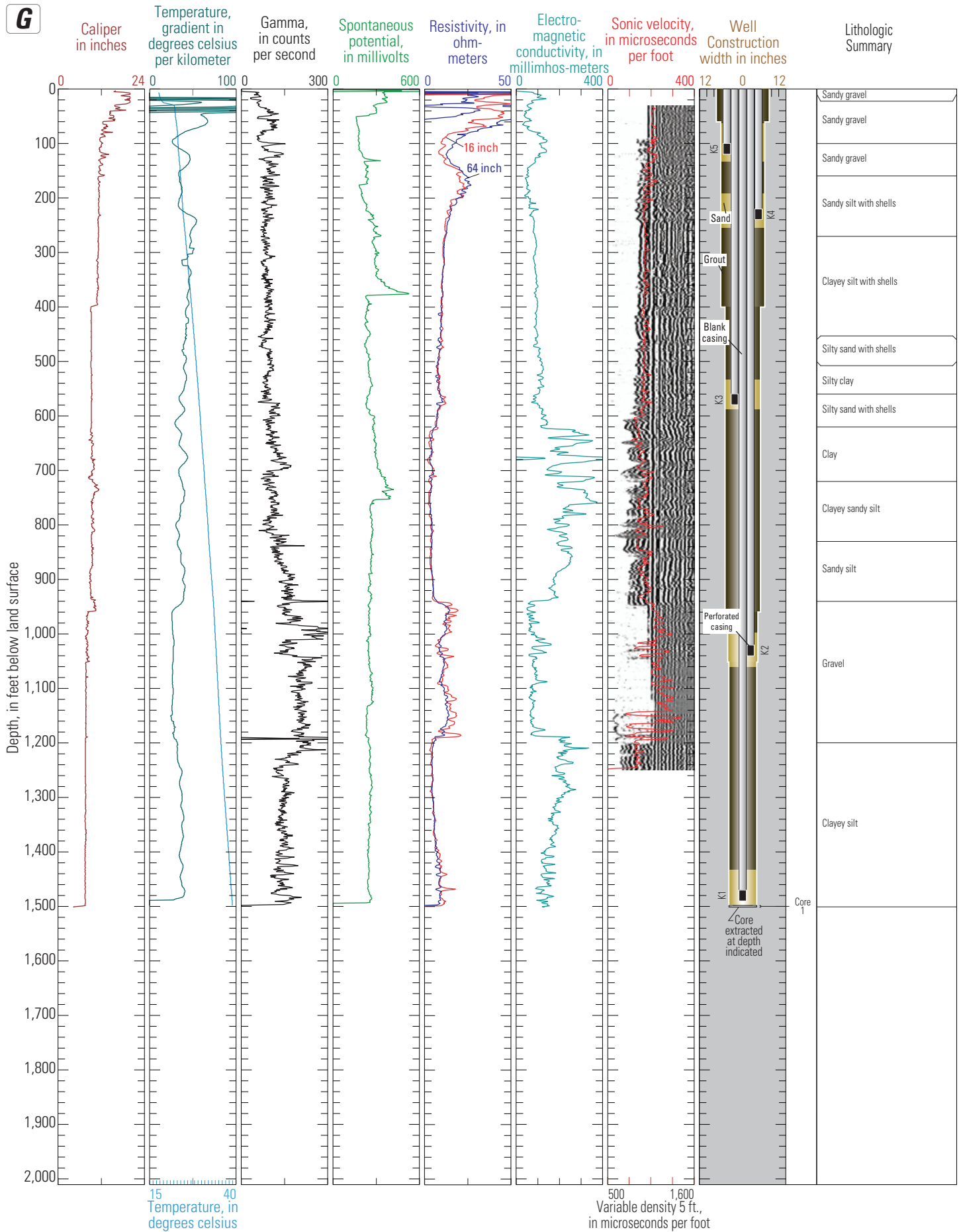
Figure 9G. Well construction diagrams and geophysical log data for caliper, temperature, natural gamma, SP, resistivity, EM, and sonic logs collected from the USGS multiple-depth monitoring-well sites in San Diego County, California, 2003-2009: (A) SDBW (B) SDOT (C) SDOR (D) SDMC (E) SDNB (F) SDEP (G) SDBP (H) SDAQ.—Continued
