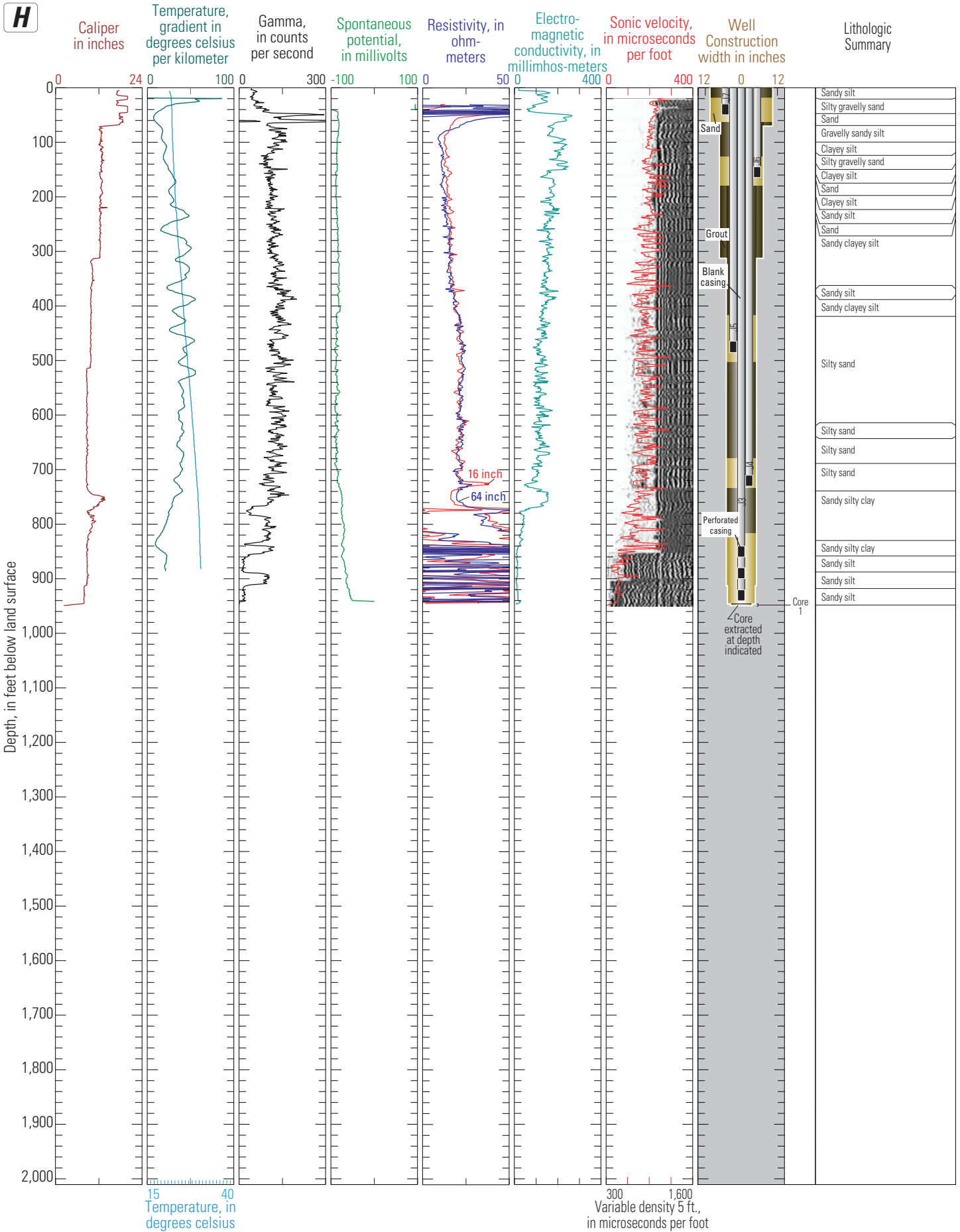
Figure 9H. Well construction diagrams and geophysical log data for caliper, temperature, natural gamma, SP, resistivity, EM, and sonic logs collected from the USGS multiple-depth monitoring-well sites in San Diego County, California, 2003-2009: (A) SDBW (B) SDOT (C) SDOR (D) SDMC (E) SDNB (F) SDEP (G) SDBP (H) SDAQ.—Continued
