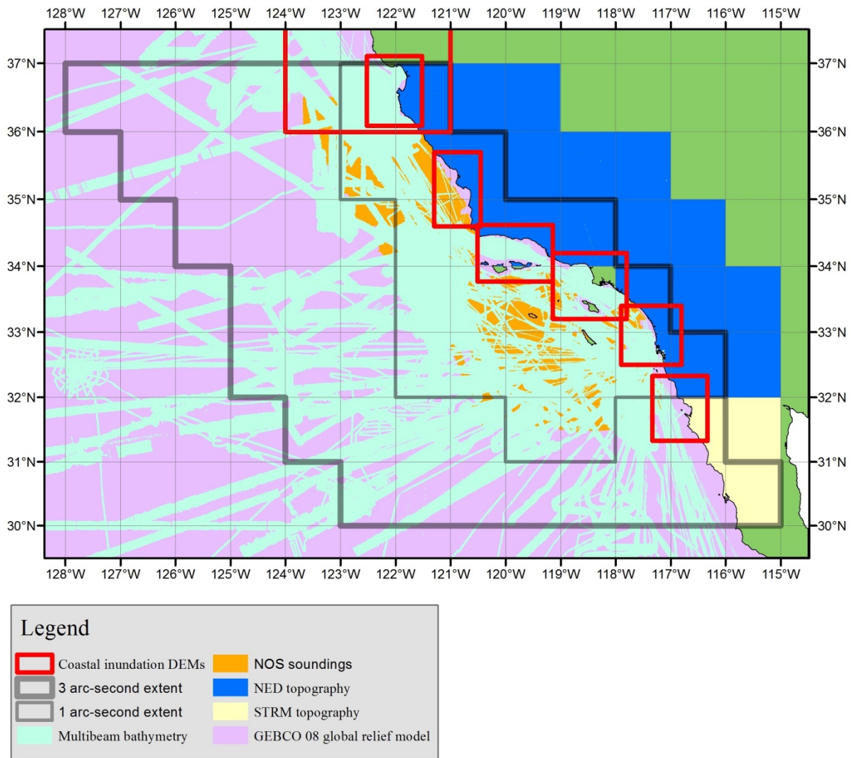
Figure 5: Principle source dataset contributions to the revised Southern California CRM.
