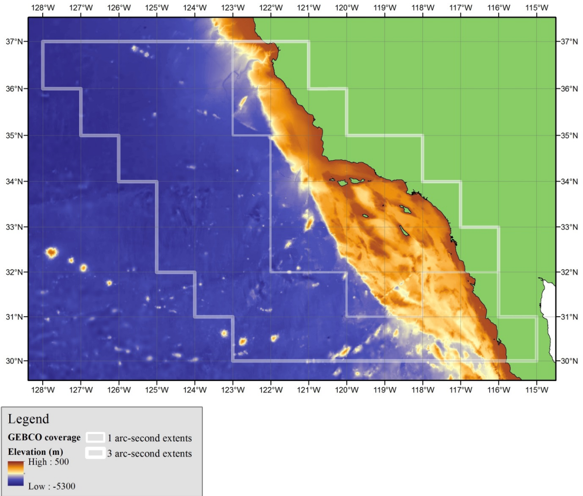
Figure 7: Shaded relief image of bathymetric data extracted from GEBCO 08.
