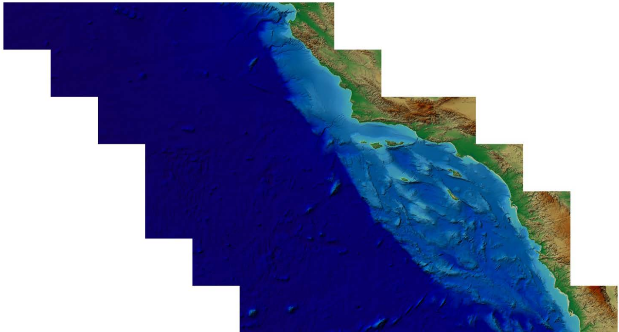
Figure 1: Shaded relief image of the Southern California CRM.
