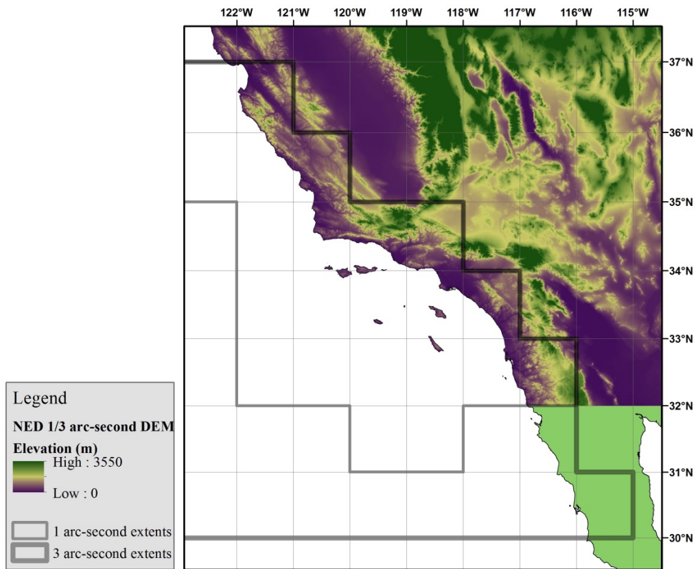
Figure 8: Shaded relief image representing the 1/3 arc-second NED topography used to build the Southern California CRM. The 1/3 arc-second DEMs are only available for the continental U.S., above 32°N; 1 arc-second data are available for regions extending outside of the U.S.
