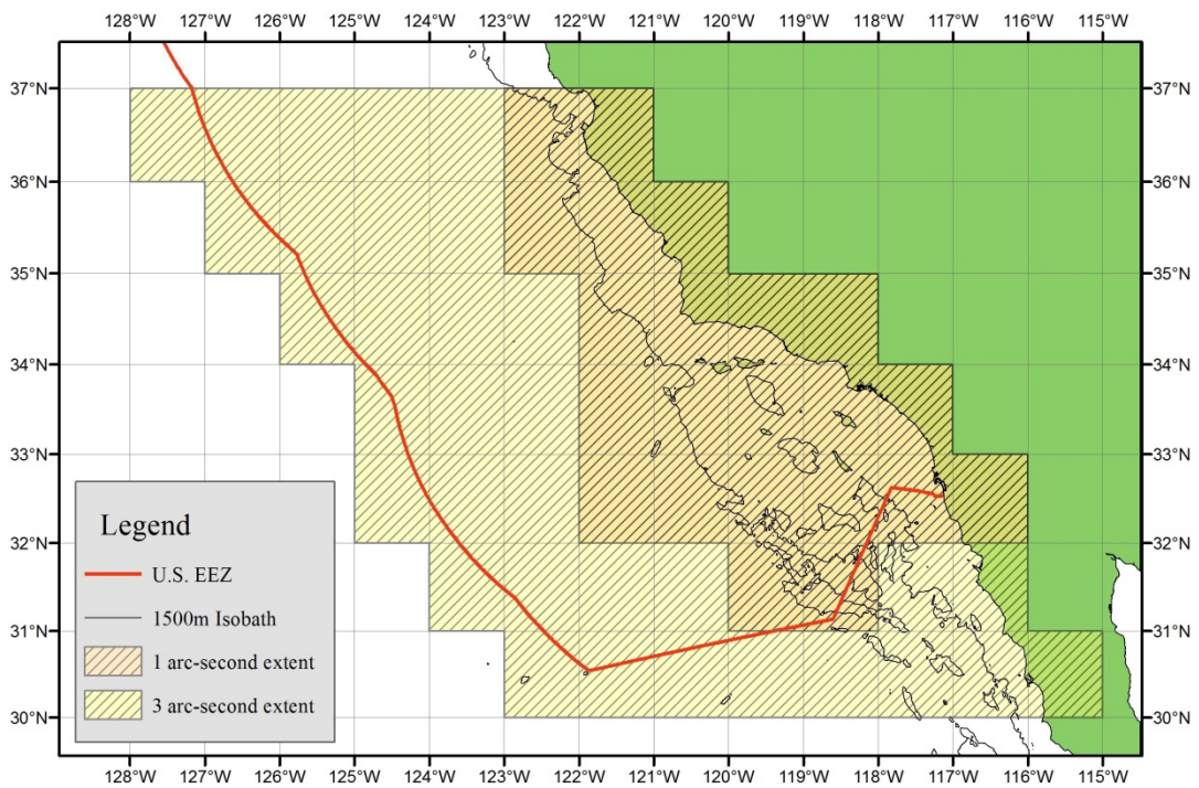
Figure 4: Extents for the revised Southern California CRM. The limit of the U.S. Exclusive Economic Zone for the Pacific Ocean is depicted in red. The 1500 meter isobath is depicted in black.
