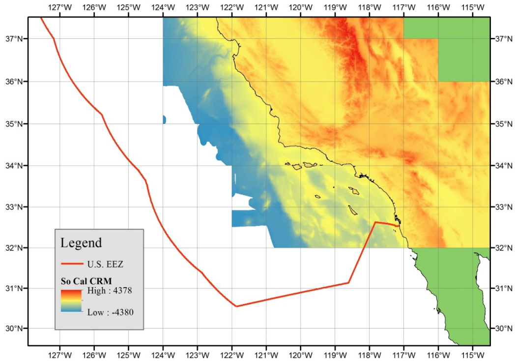
Figure 3: Color relief image of the first version of the Southern California CRM. The limit of the U.S. Exclusive Economic Zone for the Pacific Ocean is depicted in red.
