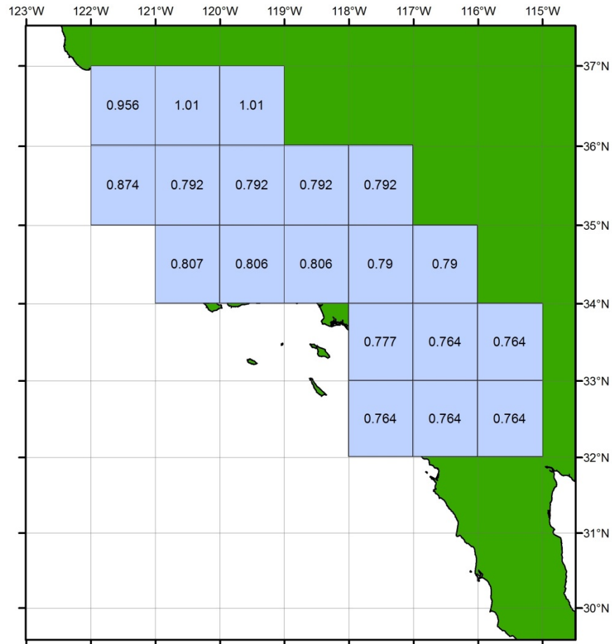
Figure 11: Constant offsets used to convert between MSL and NAVD 88 vertical datums.
