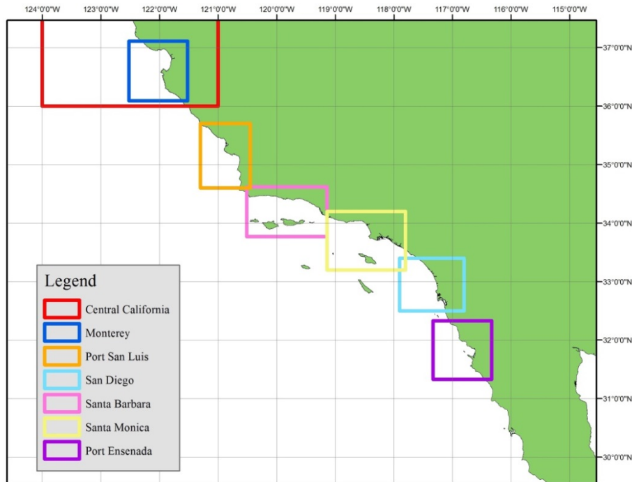
Figure 10: Coverage of high resolution integrated bathymetric and topographic DEMs developed by NGDC.
