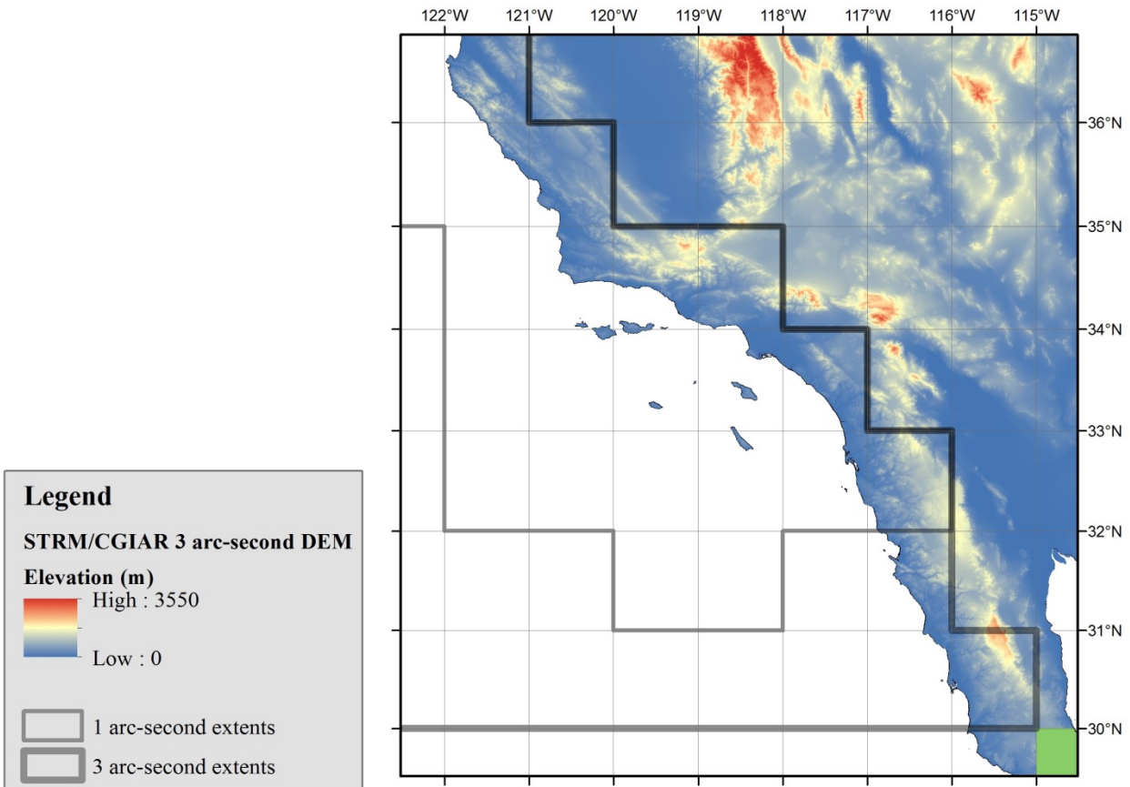
Figure 9: Shaded relief image representing the STRM/CGIAR 3 arc-second topography used to build the Southern California CRM. This dataset was clipped to only include regions not covered by the NED DEMs.
