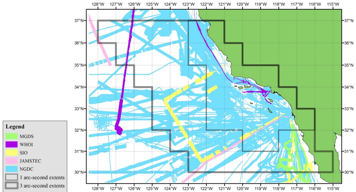
Figure 6: Multibeam coverage for the Southern California region.
