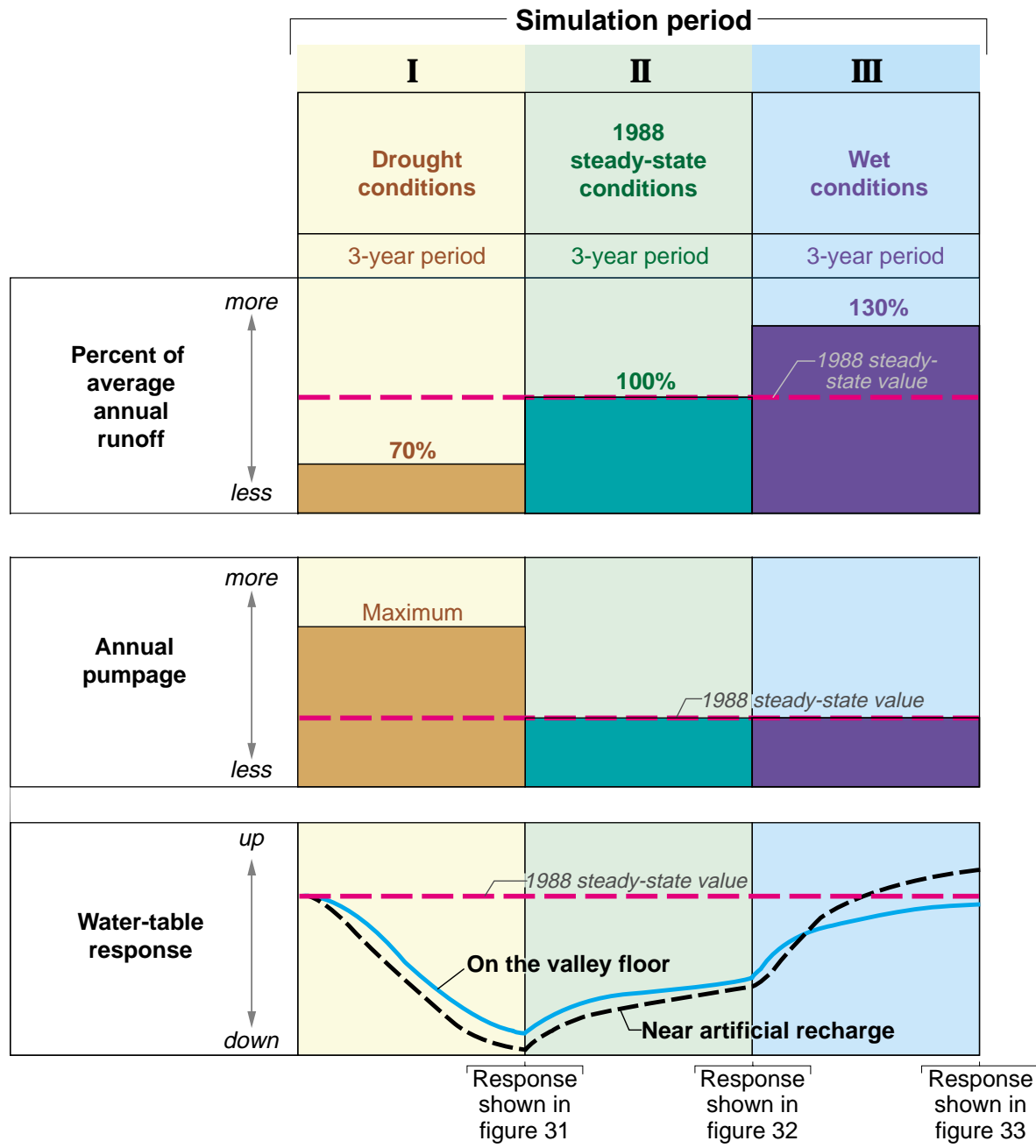
Figure 30. Diagram of water-management alternative 4 for the Owens Valley, California. Shown are changes in percent of average annual runoff, annual pumpage, and water-table response at typical locations in the valley during the 9-year simulation period. Results at the end of each 3-year period are displayed in figures 31–33.
