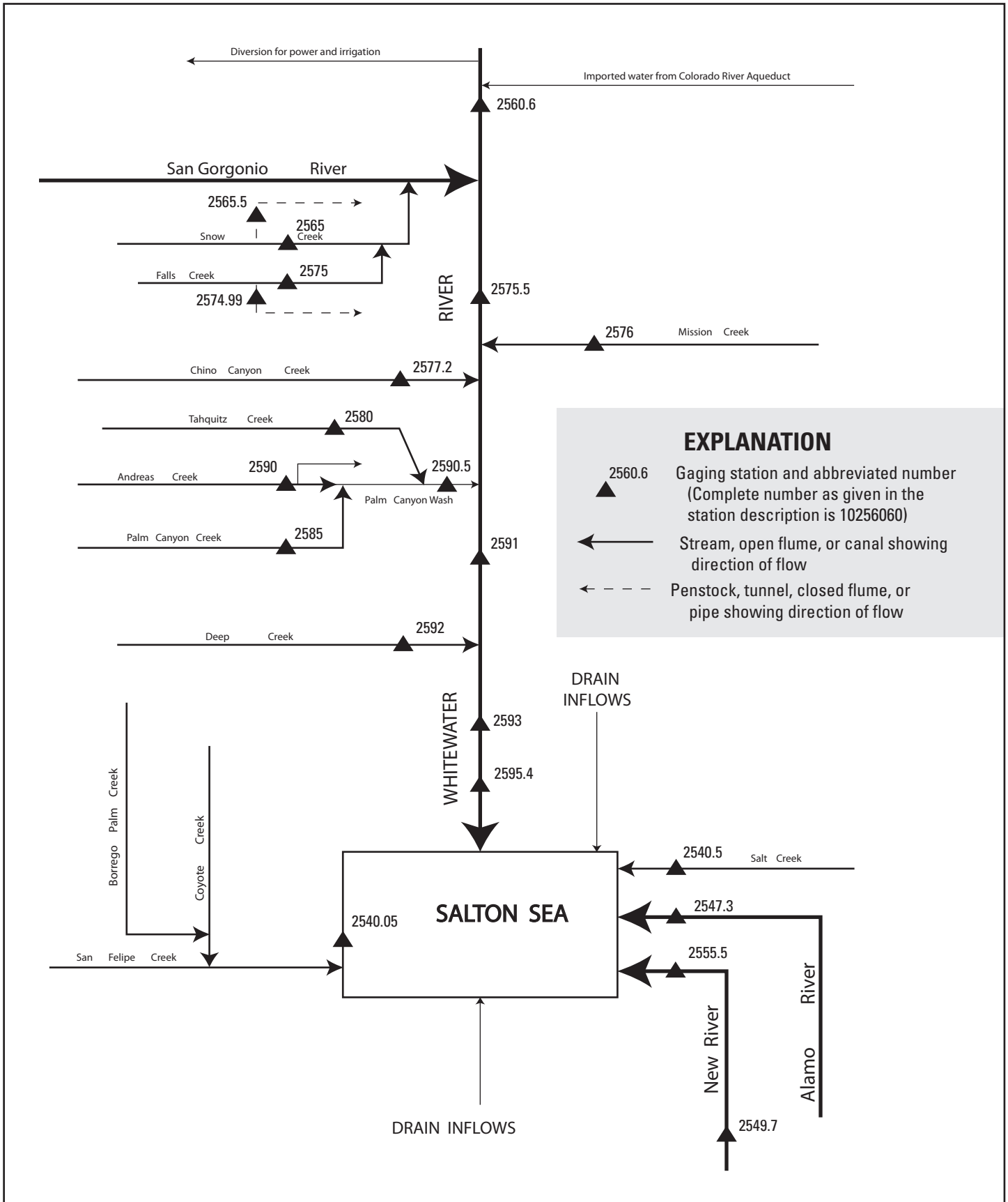
Figure showing diversions and storage in Salton Sea Basin.
