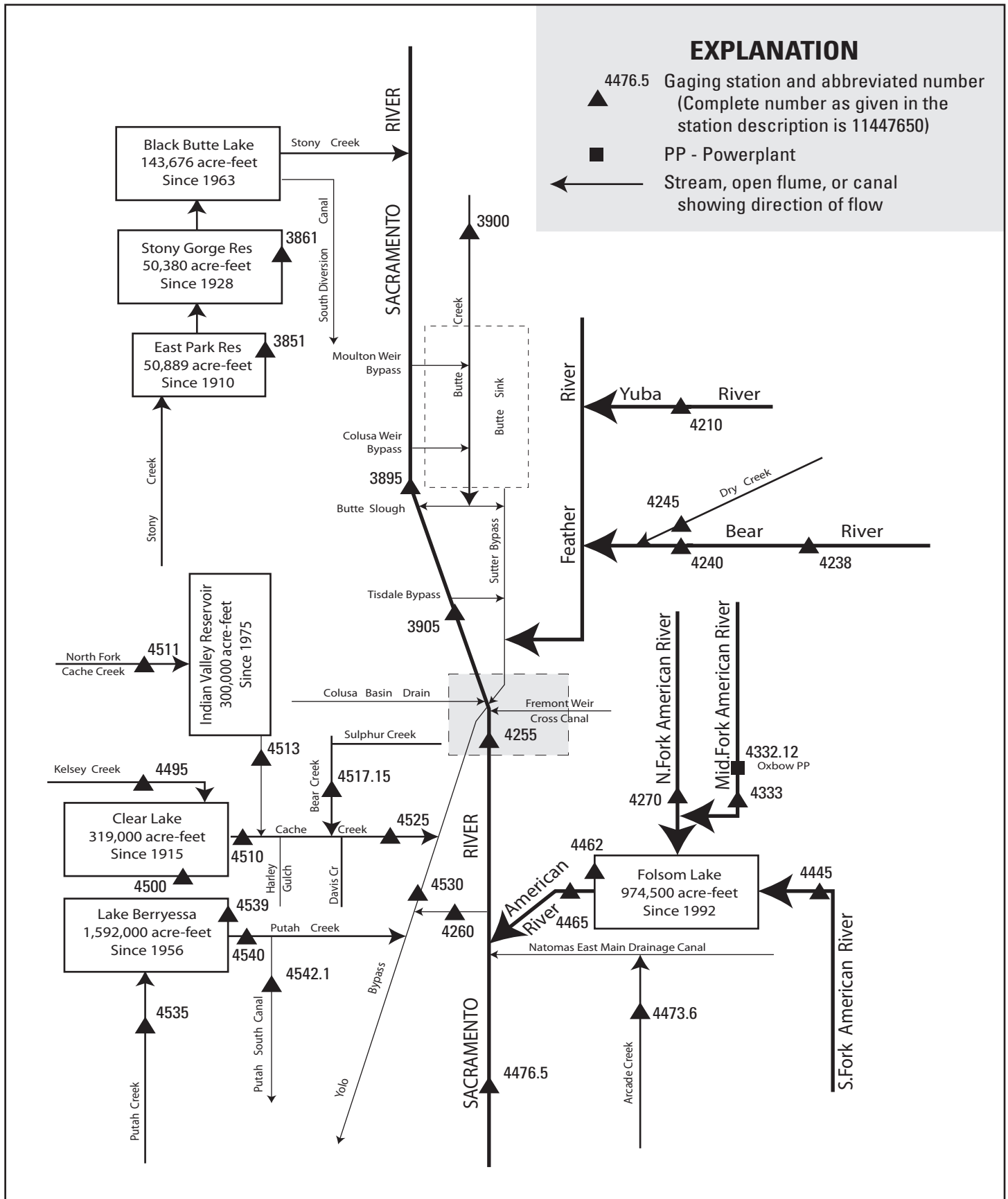
Figure showing diversions and storage in lower Sacramento River Basin.
