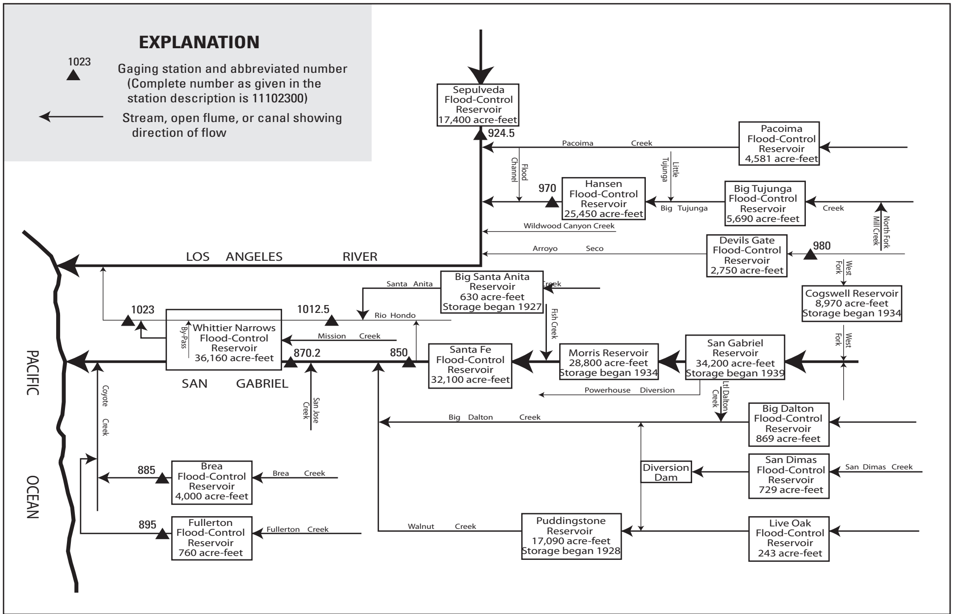
Figure showing diversions and storage in San Gabriel River and Los Angeles River Basins.
