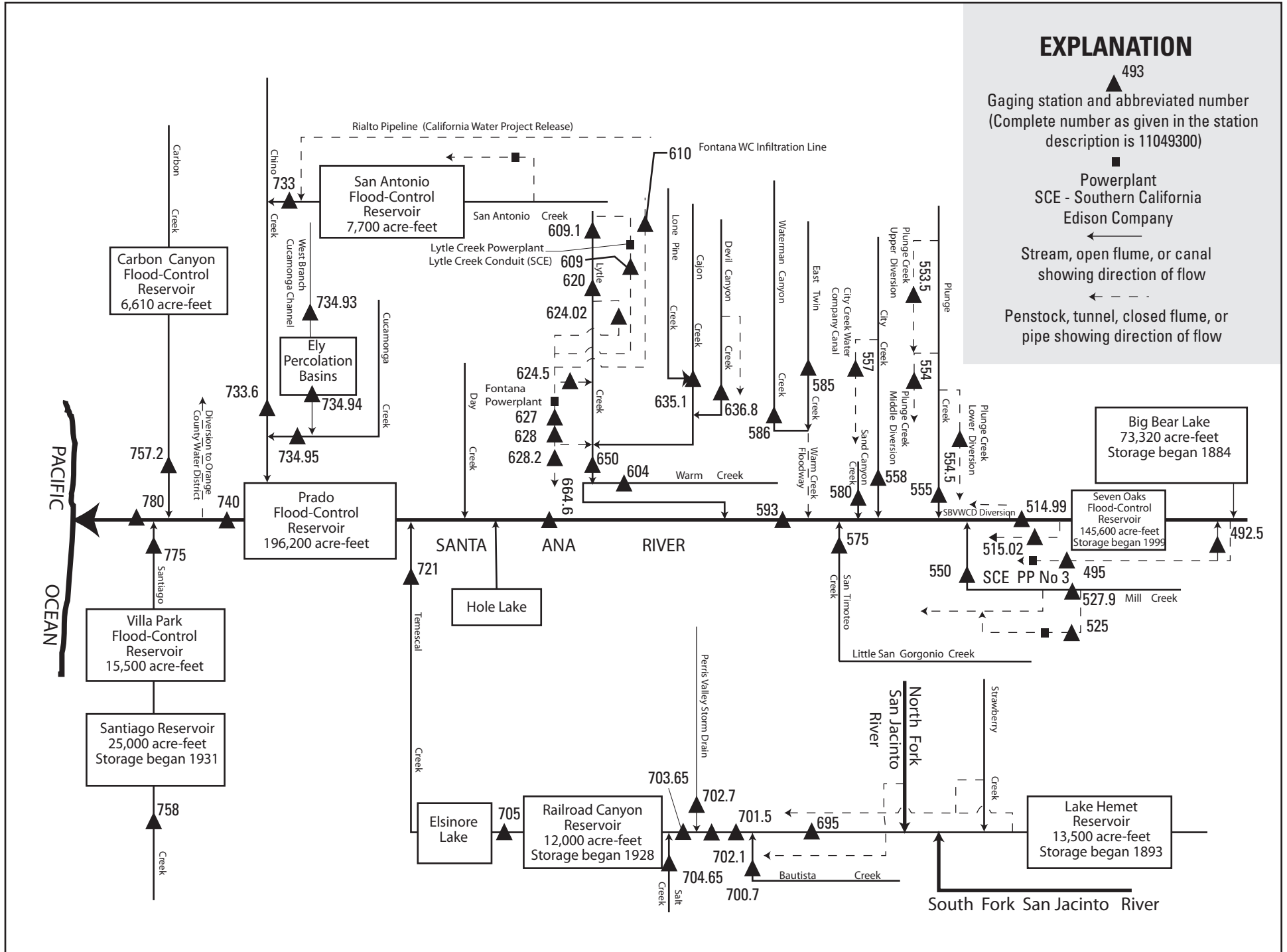
Figure showing diversions and storage in Santa Ana River Basin.
