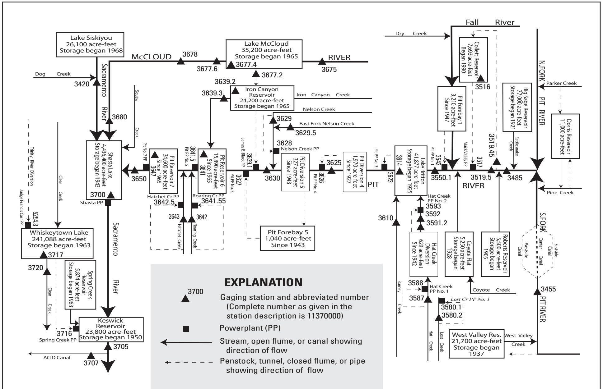
Figure showing diversions and storage in Pit River and McCloud River Basins.
