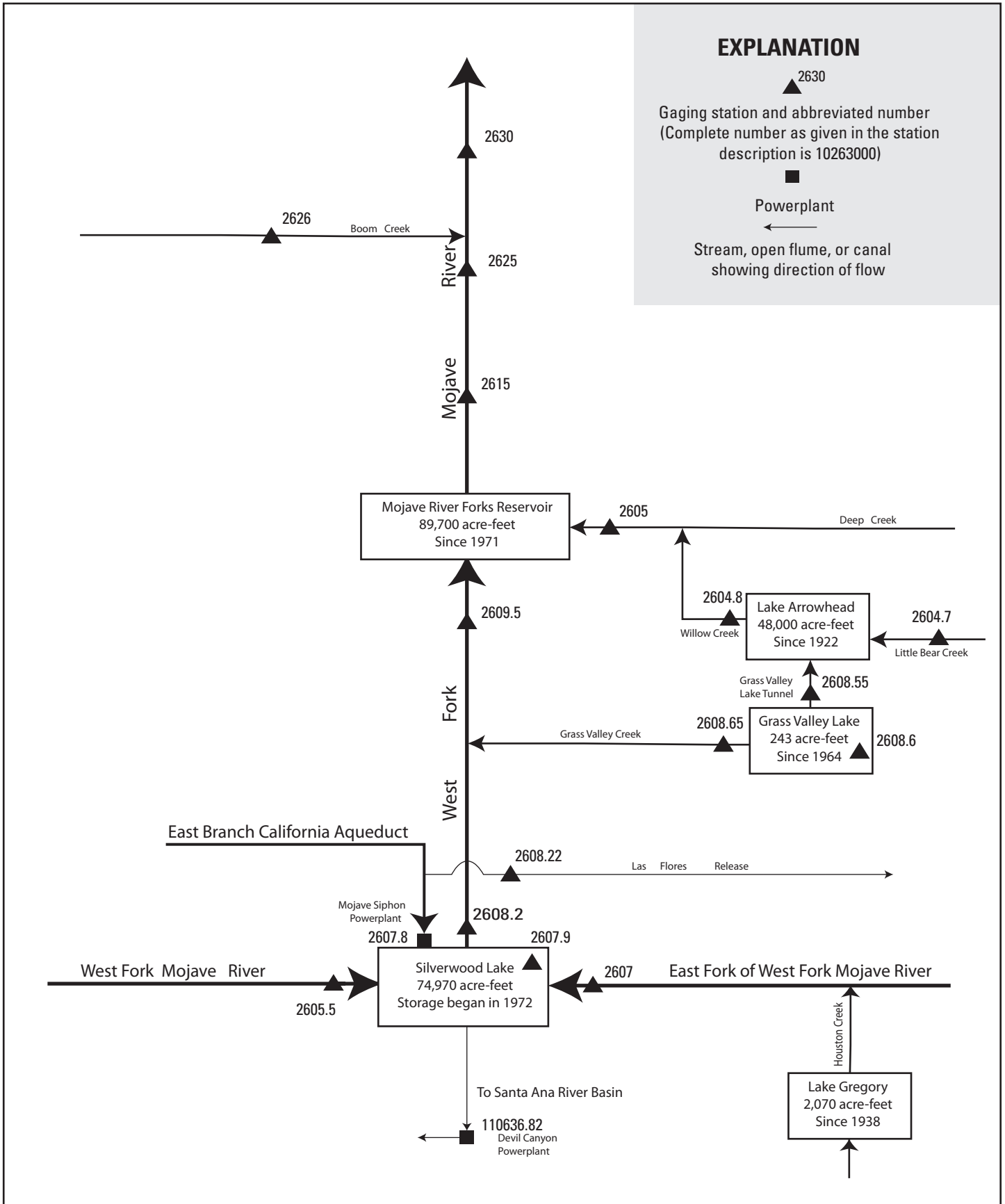
Figure showing diversions and storage in Mojave River Basin.
