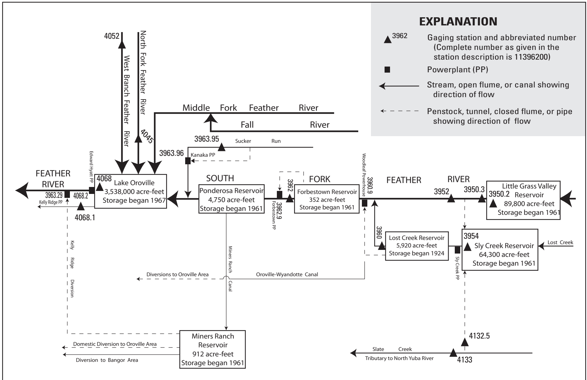
Figure showing diversions and storage in South Fork Feather River Basin.
