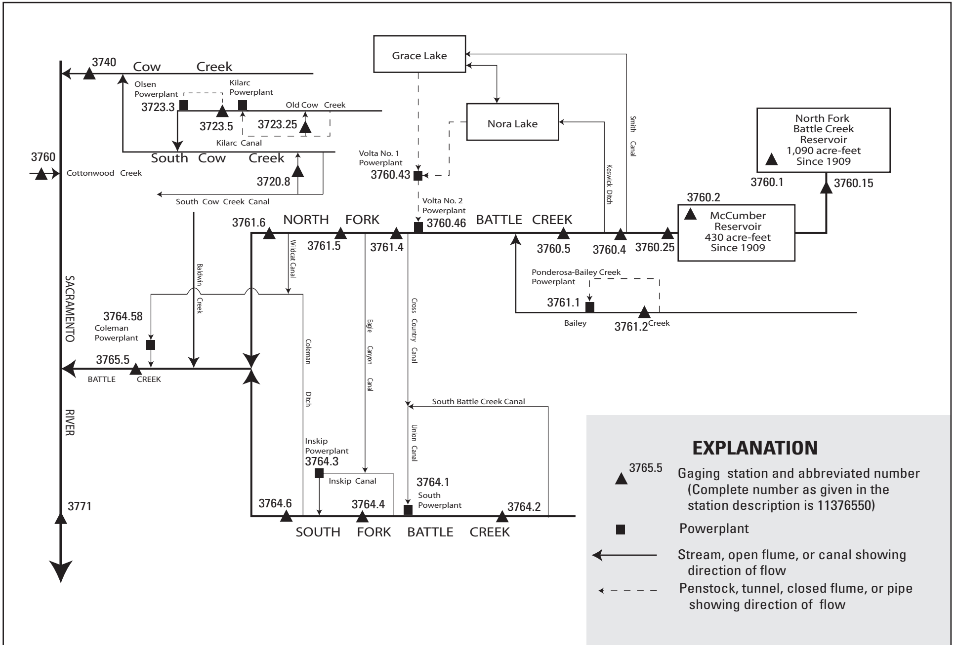
Figure showing diversions and storage in Battle Creek and Cow Creek Basins.
