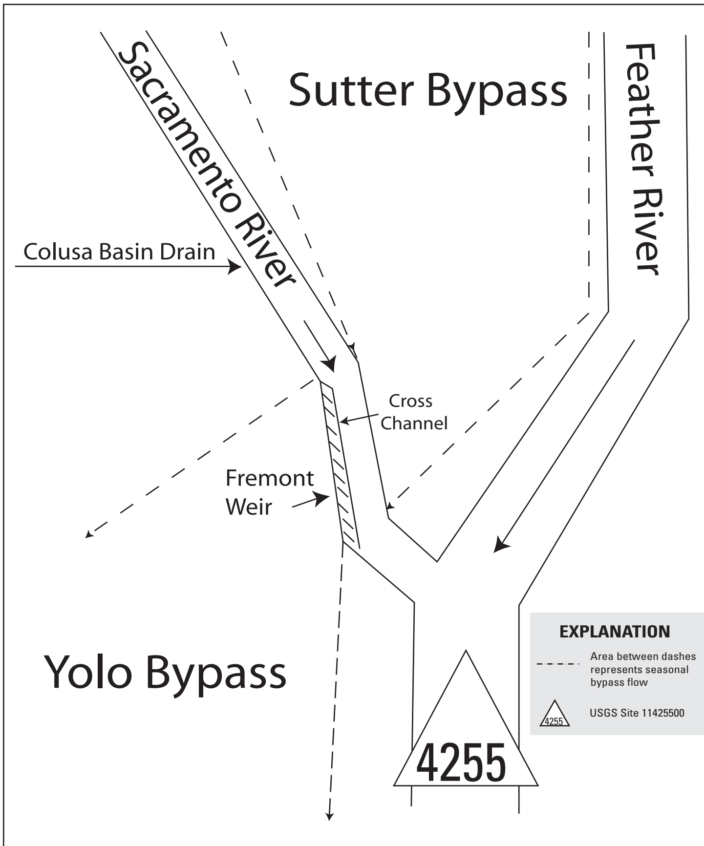
Figure showing diversions and storage in lower Sacramento River Basin, Fremont Weir.
