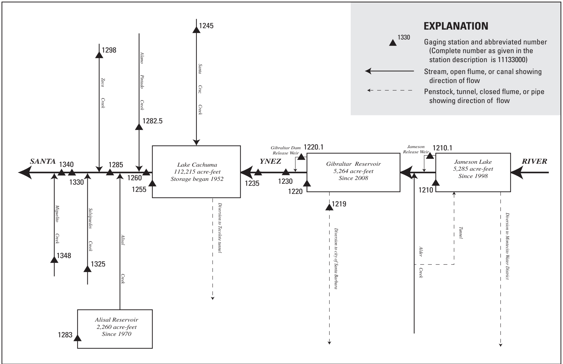
Figure showing diversions and storage in Santa Ynez River Basin.
