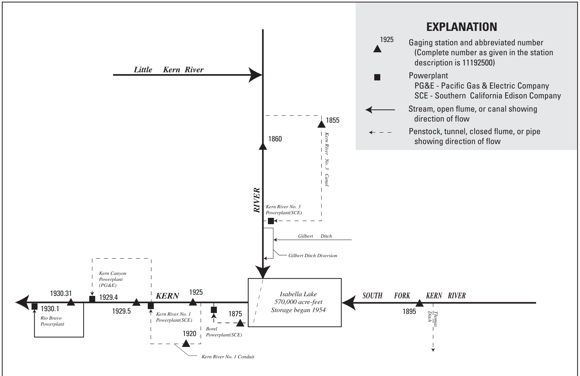
Figure showing diversions and storage in Kern River Basin.
