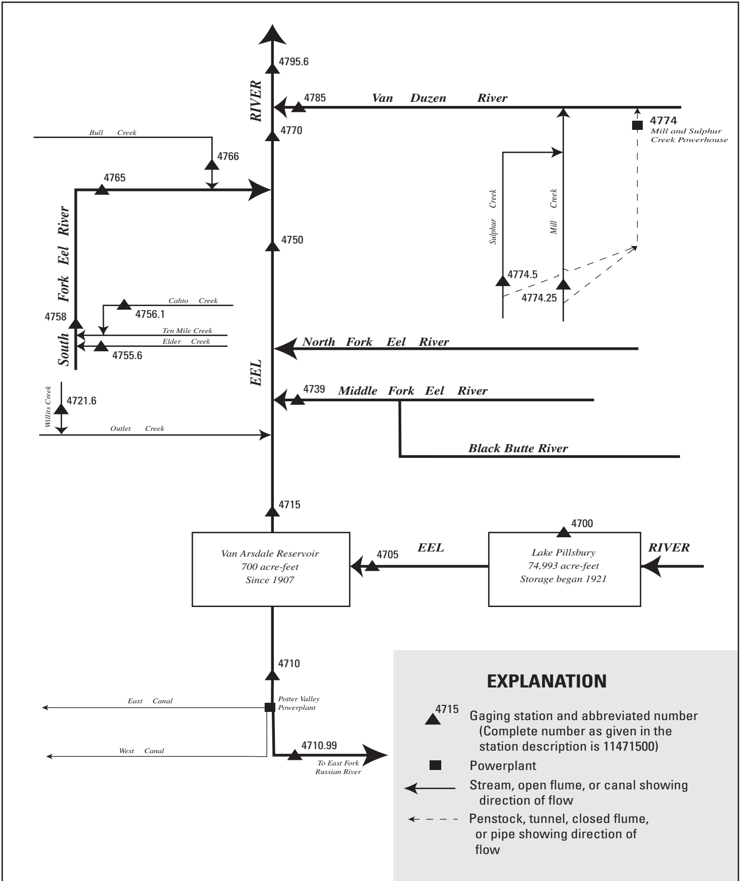
Figure showing diversions and storage in Eel River Basin.
