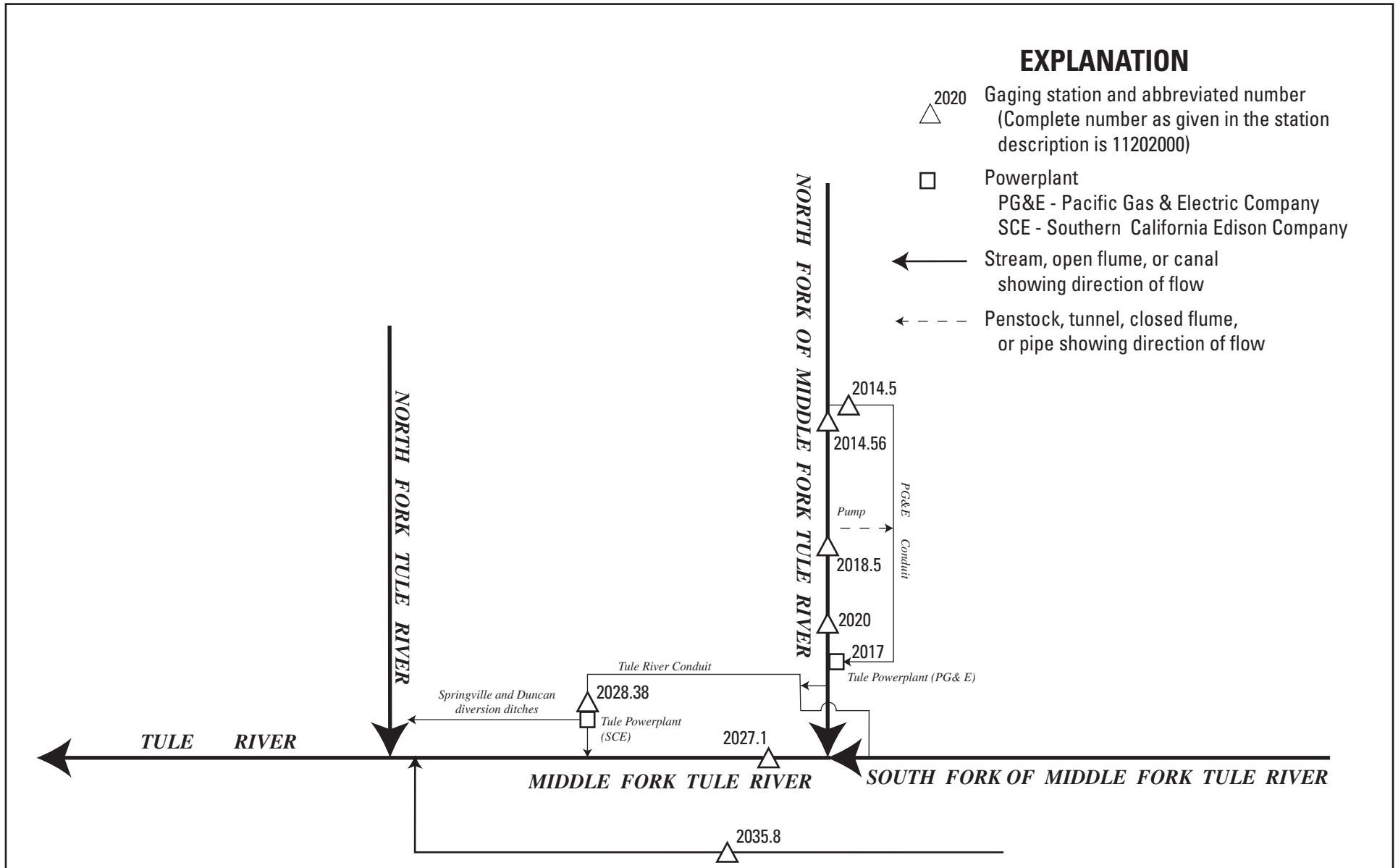
Figure showing diversions and storage in Tule River Basin.
