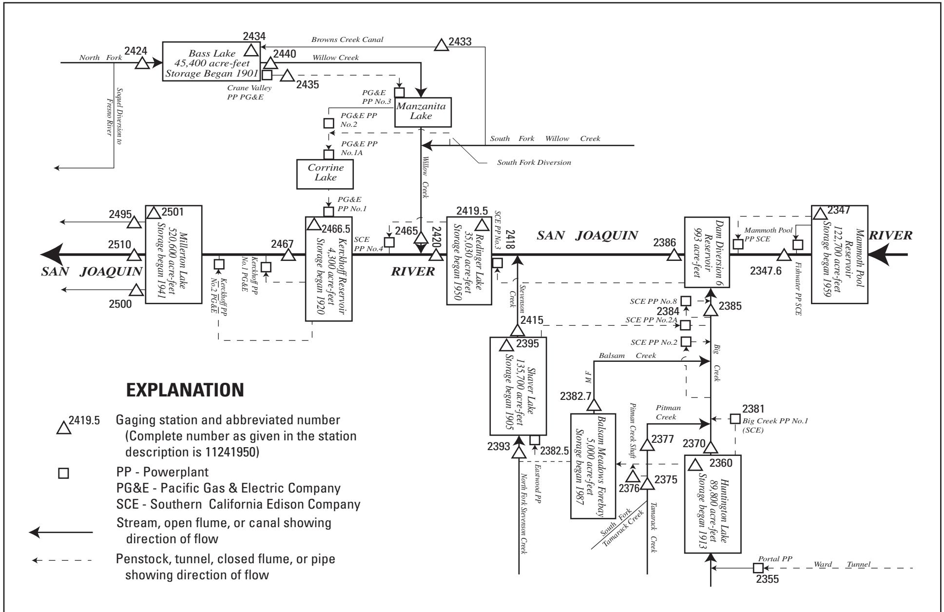
Figure showing diversions and storage in lower San Joaquin River Basin.
