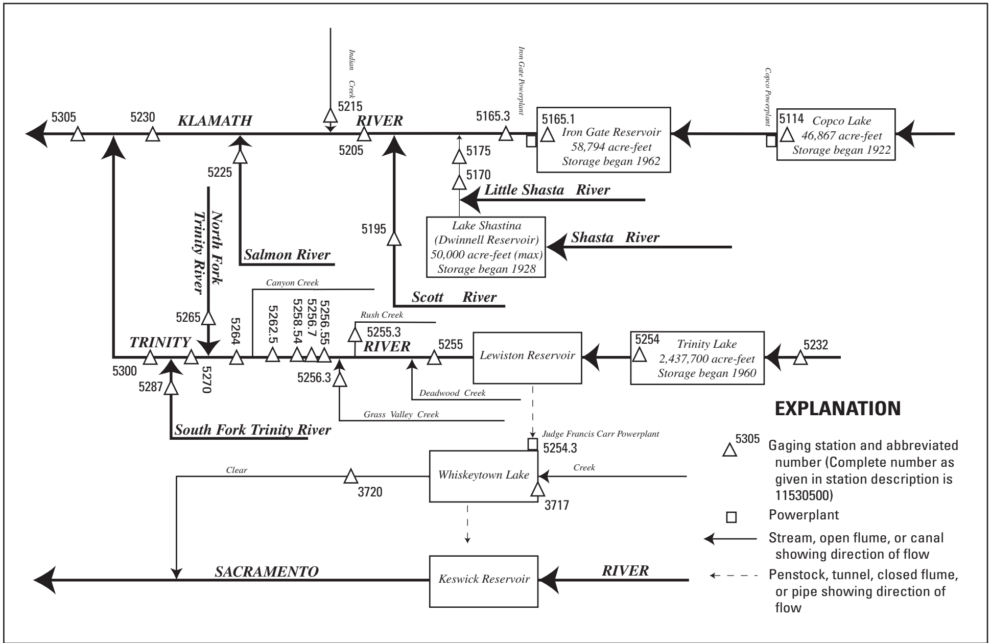
Figure showing diversions and storage in Klamath River and Trinity River Basins.
